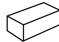
STANDARD BRICK 230MM LONG X 110MM WIDE X 76MM HIGH
