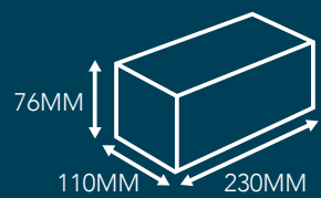
STANDARD BRICK
